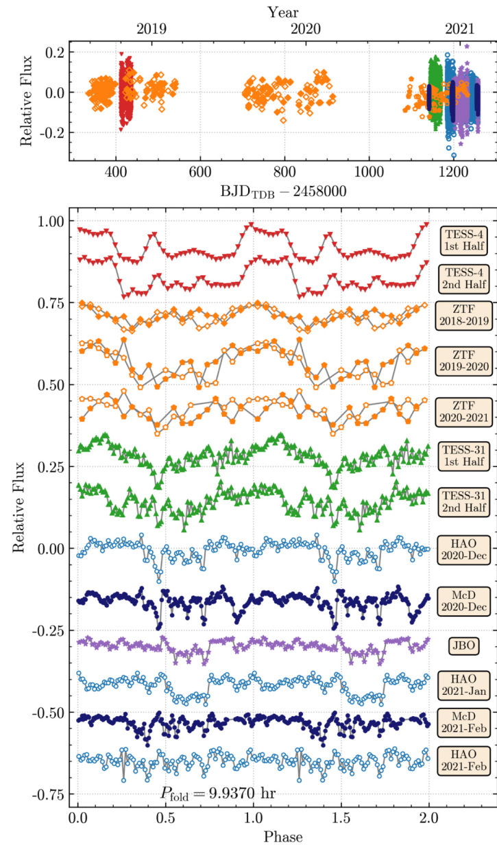
Figure 3. from Recurring Planetary Debris Transits and Circumstellar Gas around White Dwarf ZTF J0328–1219 null 2021 APJ 917 41 doi:10.3847/1538-4357/ac0822 https://dx.doi.org/10.3847/1538-4357/ac0822 © 2021. The American Astronomical Society. All rights reserved.
