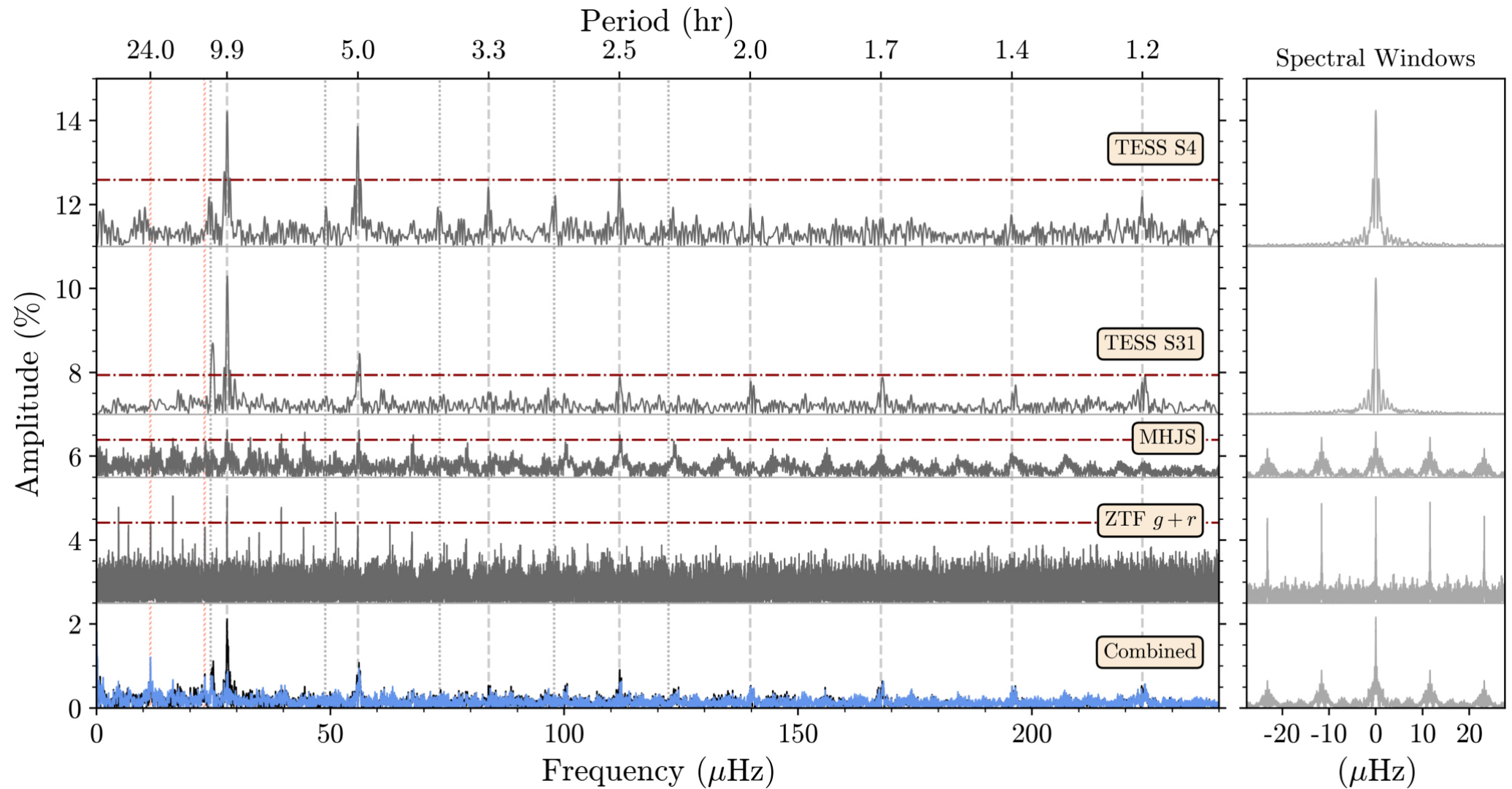
Figure 1. from Recurring Planetary Debris Transits and Circumstellar Gas around White Dwarf ZTF J0328–1219 null 2021 APJ 917 41 doi:10.3847/1538-4357/ac0822 https://dx.doi.org/10.3847/1538-4357/ac0822 © 2021. The American Astronomical Society. All rights reserved.
