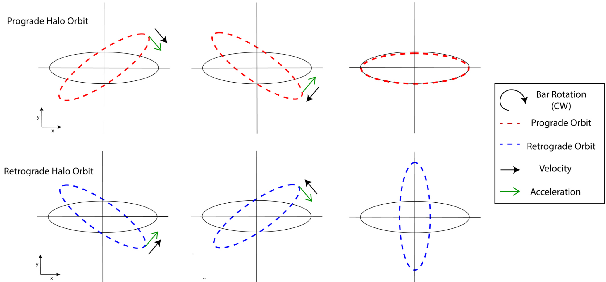
Figure 1. from The Coupling of Galactic Dark Matter Halos with Stellar Bars null 2021 APJ 915 23 doi:10.3847/1538-4357/ac004d https://dx.doi.org/10.3847/1538-4357/ac004d © 2021. The American Astronomical Society. All rights reserved.
