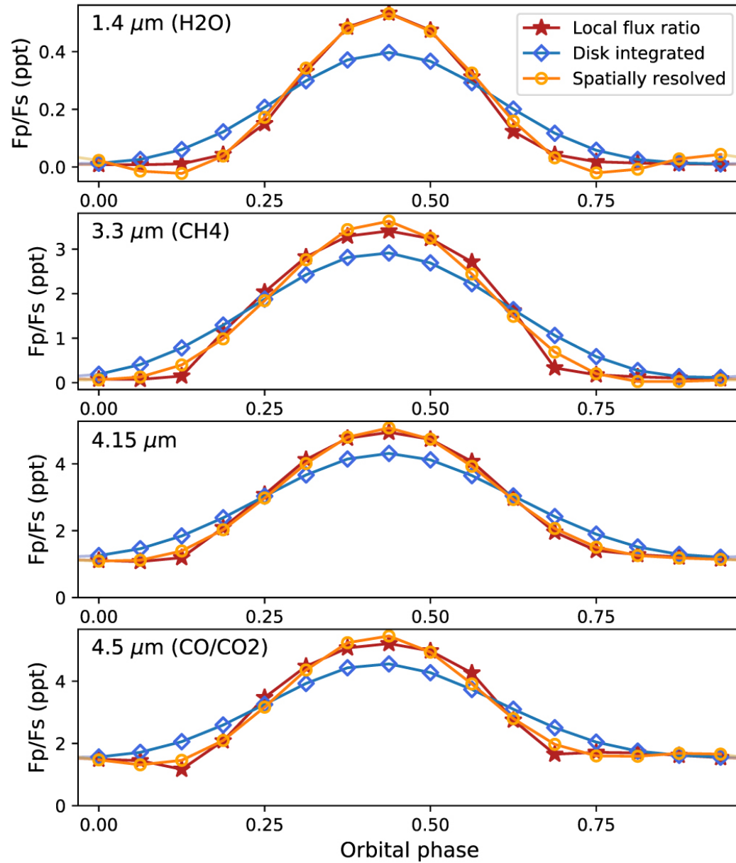
Figure 8. from Longitudinally Resolved Spectral Retrieval (ReSpect) of WASP-43b null 2021 APJ 915 45 doi:10.3847/1538-4357/abfe14 https://dx.doi.org/10.3847/1538-4357/abfe14 © 2021. The American Astronomical Society. All rights reserved.
