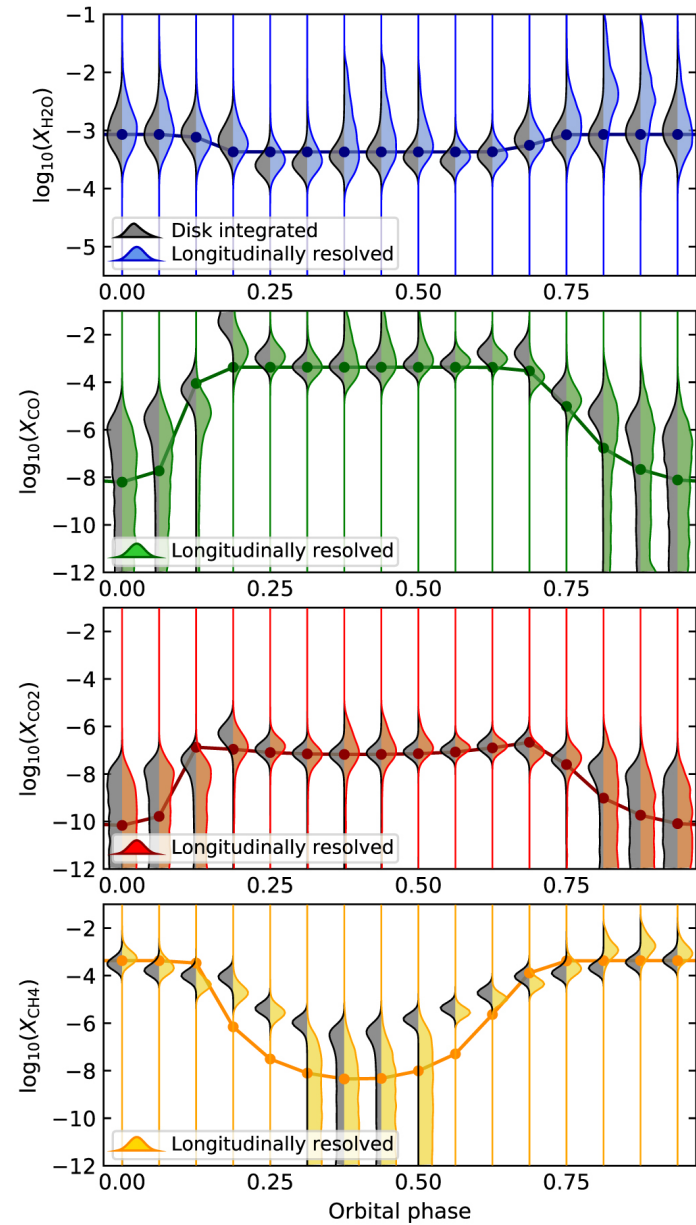
Figure 7. from Longitudinally Resolved Spectral Retrieval (ReSpect) of WASP-43b null 2021 APJ 915 45 doi:10.3847/1538-4357/abfe14 https://dx.doi.org/10.3847/1538-4357/abfe14 © 2021. The American Astronomical Society. All rights reserved.
