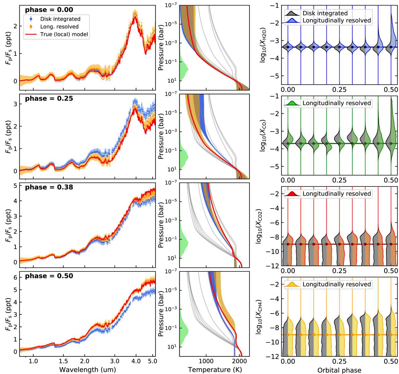
Figure 5. from Longitudinally Resolved Spectral Retrieval (ReSpect) of WASP-43b null 2021 APJ 915 45 doi:10.3847/1538-4357/abfe14 https://dx.doi.org/10.3847/1538-4357/abfe14
