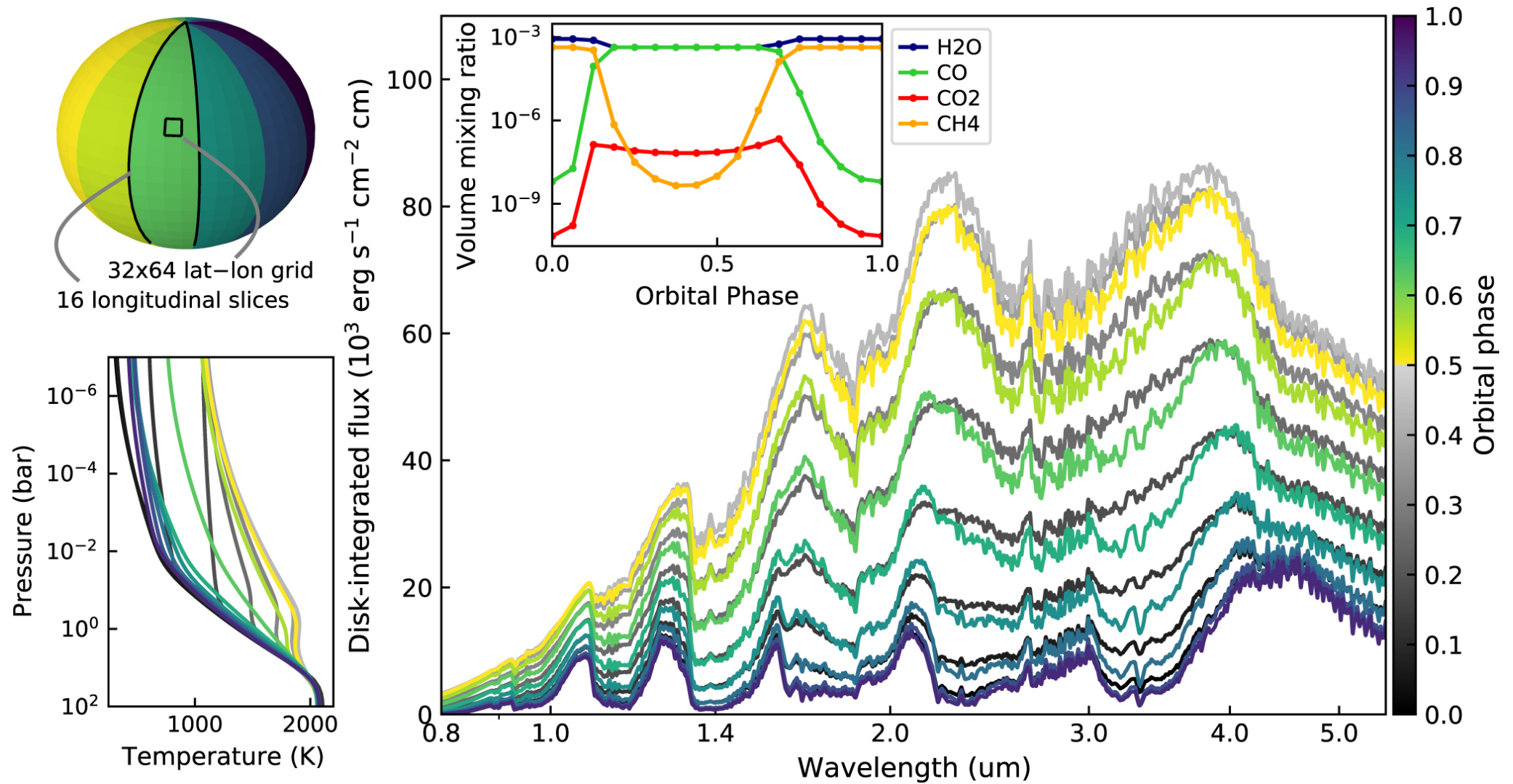
Figure 4. from Longitudinally Resolved Spectral Retrieval (ReSpect) of WASP-43b null 2021 APJ 915 45 doi:10.3847/1538-4357/abfe14 https://dx.doi.org/10.3847/1538-4357/abfe14 © 2021. The American Astronomical Society. All rights reserved.
