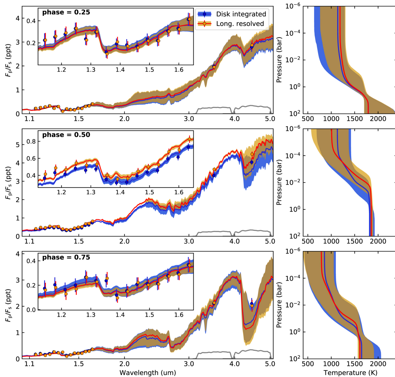
Figure 1. from Longitudinally Resolved Spectral Retrieval (ReSpect) of WASP-43b null 2021 APJ 915 45 doi:10.3847/1538-4357/abfe14 https://dx.doi.org/10.3847/1538-4357/abfe14 © 2021. The American Astronomical Society. All rights reserved.
