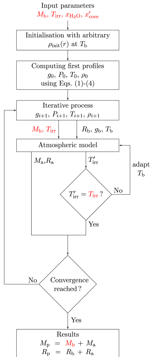
Figure 9. from Mass–Radius Relationships for Irradiated Ocean Planets null 2021 APJ 914 84 doi:10.3847/1538-4357/abfa99 https://dx.doi.org/10.3847/1538-4357/abfa99 © 2021. The American Astronomical Society. All rights reserved.
