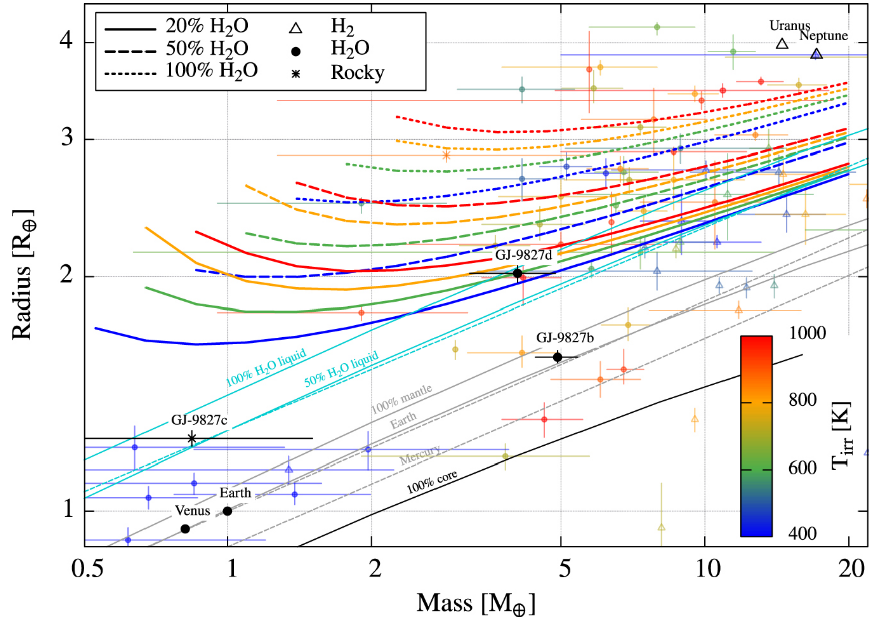
Figure 8. from Mass–Radius Relationships for Irradiated Ocean Planets null 2021 APJ 914 84 doi:10.3847/1538-4357/abfa99 https://dx.doi.org/10.3847/1538-4357/abfa99 © 2021. The American Astronomical Society. All rights reserved.
