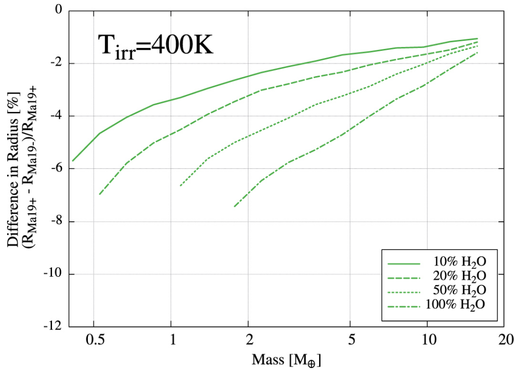
Figure 6. from Mass–Radius Relationships for Irradiated Ocean Planets null 2021 APJ 914 84 doi:10.3847/1538-4357/abfa99 https://dx.doi.org/10.3847/1538-4357/abfa99 © 2021. The American Astronomical Society. All rights reserved.
