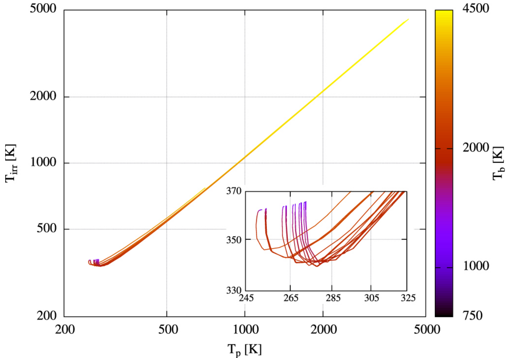
Figure 4. from Mass–Radius Relationships for Irradiated Ocean Planets null 2021 APJ 914 84 doi:10.3847/1538-4357/abfa99 https://dx.doi.org/10.3847/1538-4357/abfa99 © 2021. The American Astronomical Society. All rights reserved.
