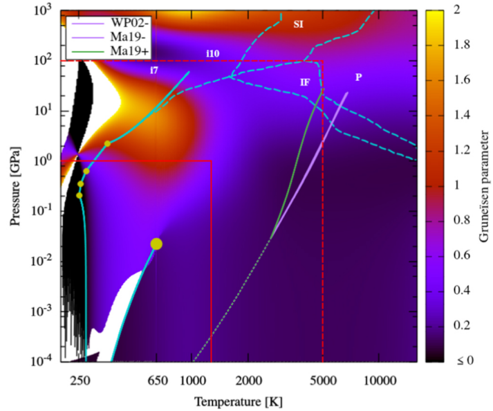
Figure 3. from Mass–Radius Relationships for Irradiated Ocean Planets null 2021 APJ 914 84 doi:10.3847/1538-4357/abfa99 https://dx.doi.org/10.3847/1538-4357/abfa99 © 2021. The American Astronomical Society. All rights reserved.
