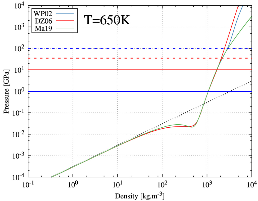
Figure 2. from Mass–Radius Relationships for Irradiated Ocean Planets null 2021 APJ 914 84 doi:10.3847/1538-4357/abfa99 https://dx.doi.org/10.3847/1538-4357/abfa99 © 2021. The American Astronomical Society. All rights reserved.
