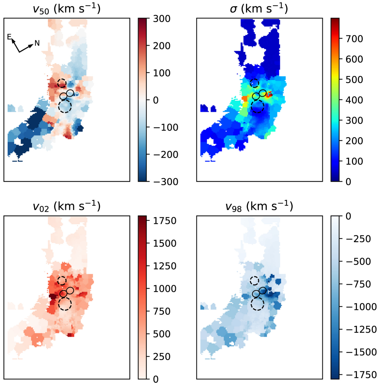
Figure 7. from KCWI Observations of the Extended Nebulae in Mrk 273 null 2021 APJ 914 17 doi:10.3847/1538-4357/abf4da https://dx.doi.org/10.3847/1538-4357/abf4da © 2021. The American Astronomical Society. All rights reserved.
