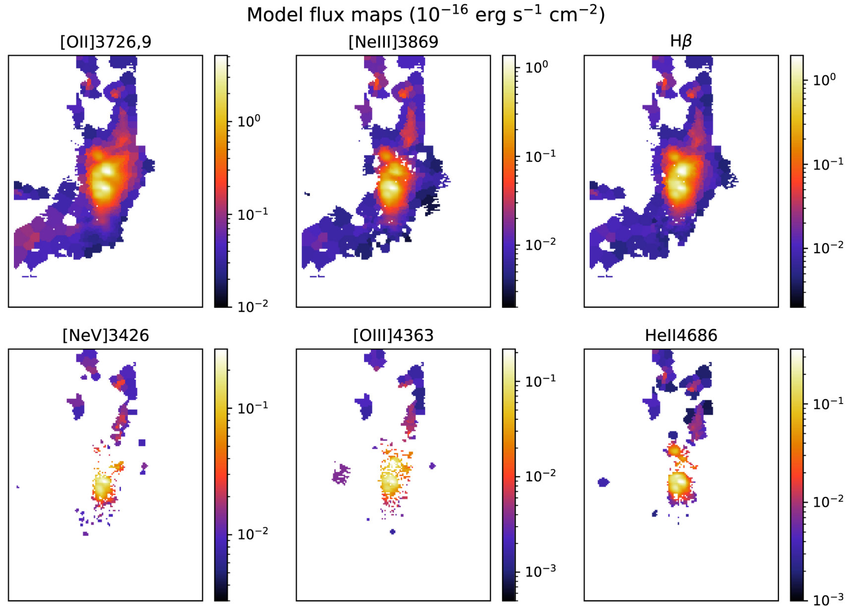
Figure 6. from KCWI Observations of the Extended Nebulae in Mrk 273 null 2021 APJ 914 17 doi:10.3847/1538-4357/abf4da https://dx.doi.org/10.3847/1538-4357/abf4da © 2021. The American Astronomical Society. All rights reserved.
