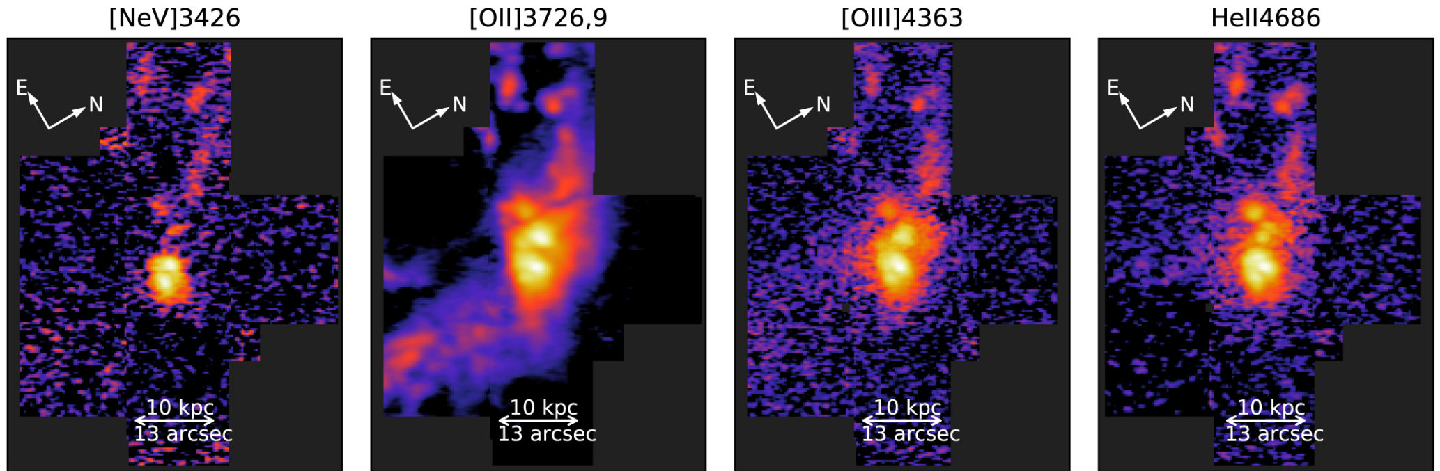
Figure 4. from KCWI Observations of the Extended Nebulae in Mrk 273 null 2021 APJ 914 17 doi:10.3847/1538-4357/abf4da https://dx.doi.org/10.3847/1538-4357/abf4da © 2021. The American Astronomical Society. All rights reserved.
