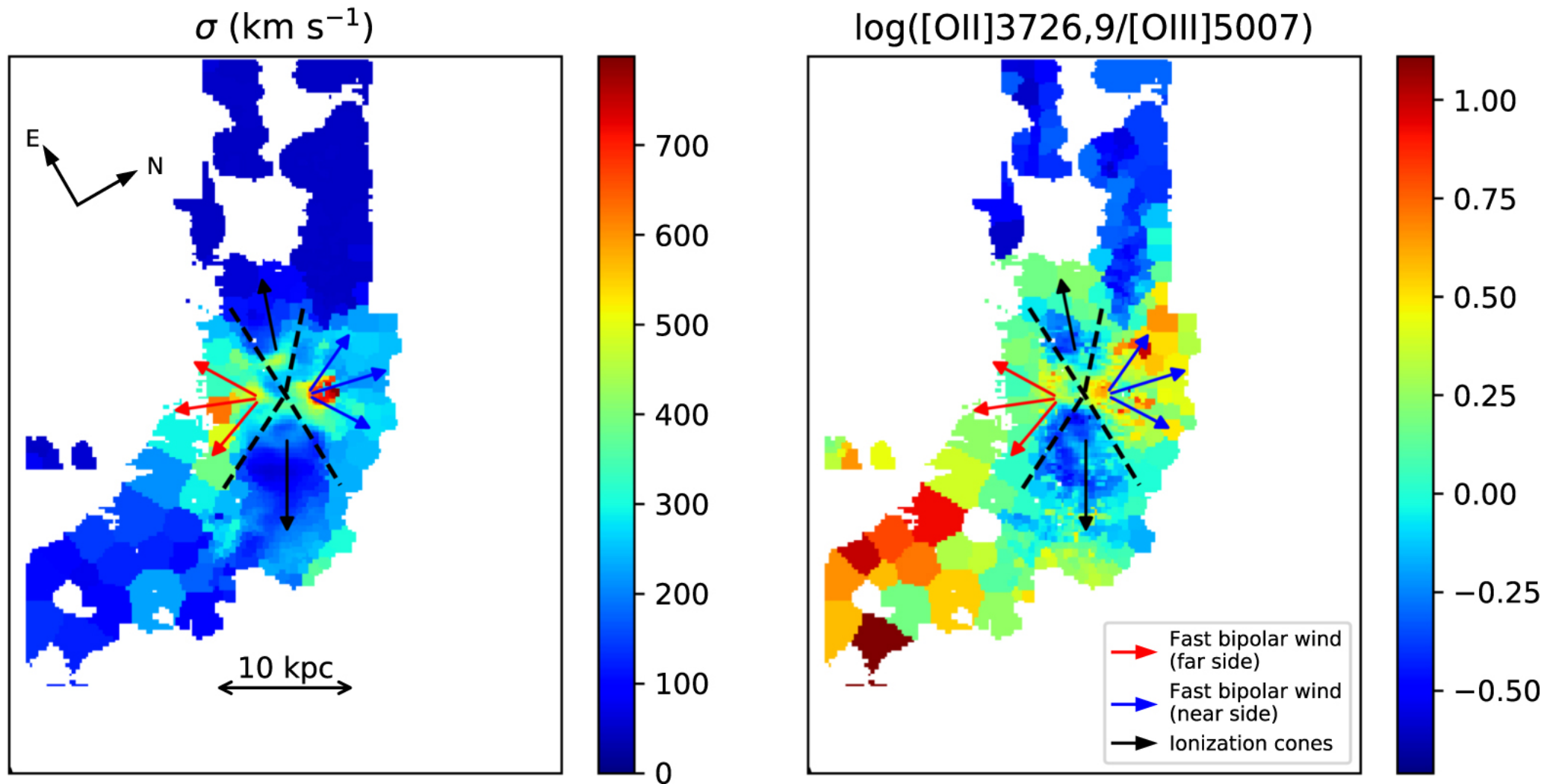
Figure 16. from KCWI Observations of the Extended Nebulae in Mrk 273 null 2021 APJ 914 17 doi:10.3847/1538-4357/abf4da https://dx.doi.org/10.3847/1538-4357/abf4da © 2021. The American Astronomical Society. All rights reserved.
