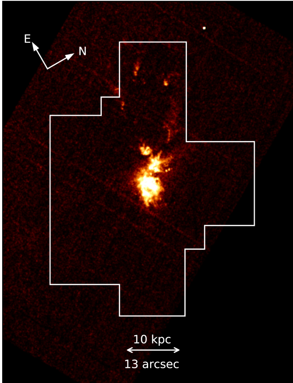
Figure 1. from KCWI Observations of the Extended Nebulae in Mrk 273 null 2021 APJ 914 17 doi:10.3847/1538-4357/abf4da https://dx.doi.org/10.3847/1538-4357/abf4da © 2021. The American Astronomical Society. All rights reserved.
