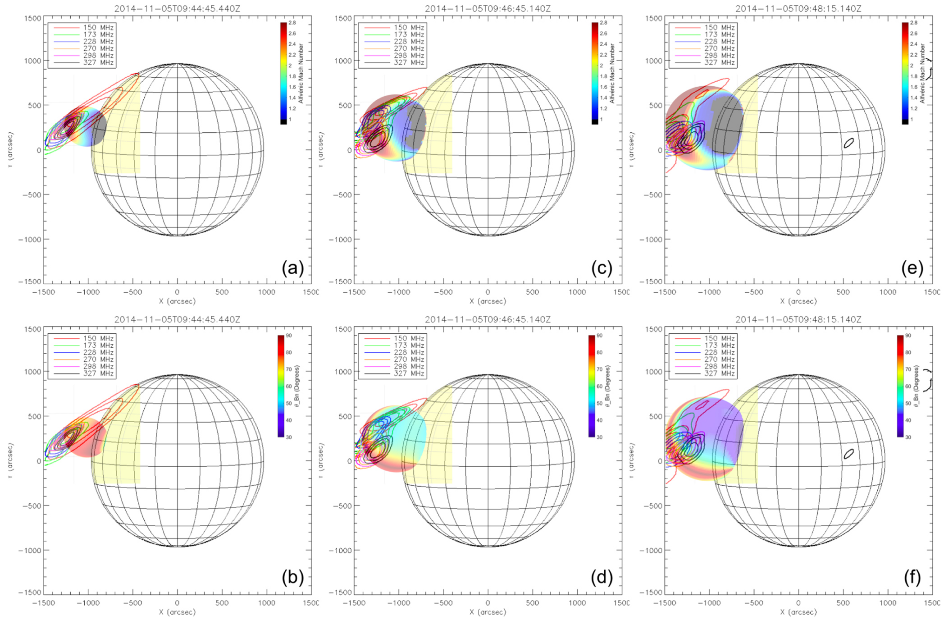
Figure 8. from Coronal Conditions for the Occurrence of Type II Radio Bursts null 2021 APJ 913 99 doi:10.3847/1538-4357/abf435 https://dx.doi.org/10.3847/1538-4357/abf435
