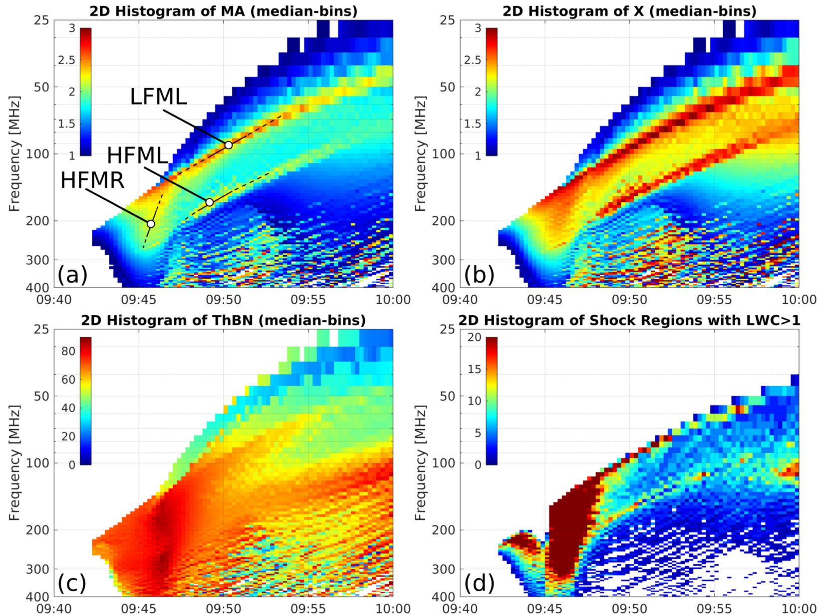
Figure 7. from Coronal Conditions for the Occurrence of Type II Radio Bursts null 2021 APJ 913 99 doi:10.3847/1538-4357/abf435 https://dx.doi.org/10.3847/1538-4357/abf435
