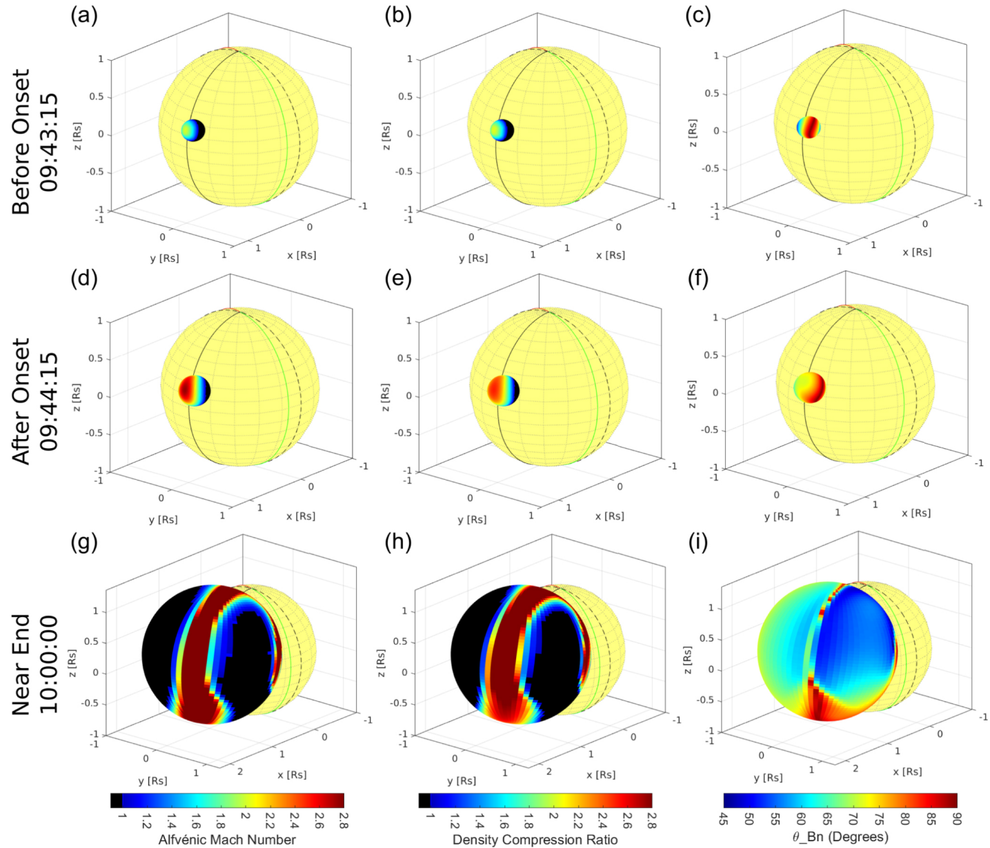
Figure 6. from Coronal Conditions for the Occurrence of Type II Radio Bursts null 2021 APJ 913 99 doi:10.3847/1538-4357/abf435 https://dx.doi.org/10.3847/1538-4357/abf435 © 2021. The Author(s). Published by the American Astronomical Society.
