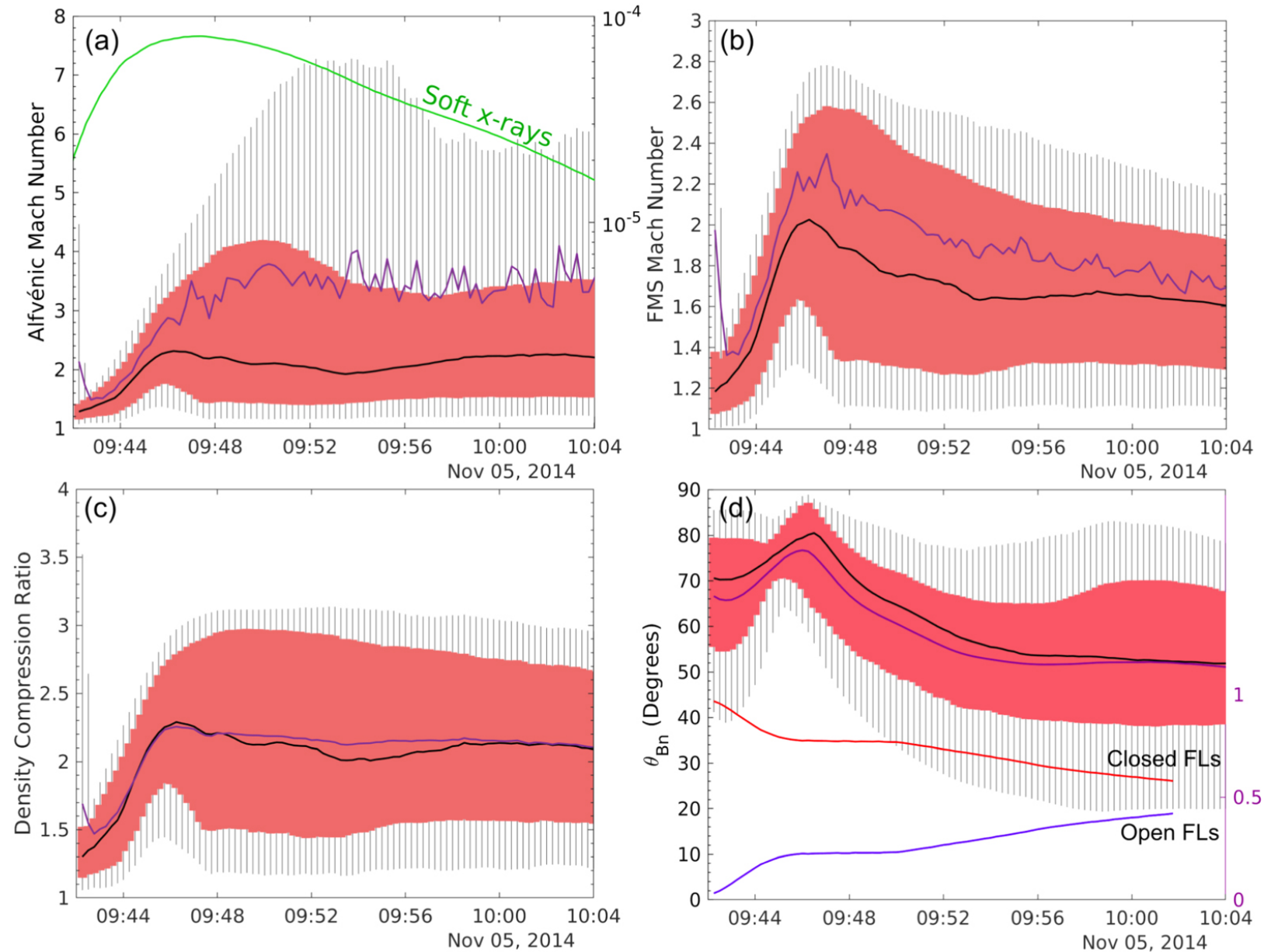
Figure 5. from Coronal Conditions for the Occurrence of Type II Radio Bursts null 2021 APJ 913 99 doi:10.3847/1538-4357/abf435 https://dx.doi.org/10.3847/1538-4357/abf435 © 2021. The Author(s). Published by the American Astronomical Society.
