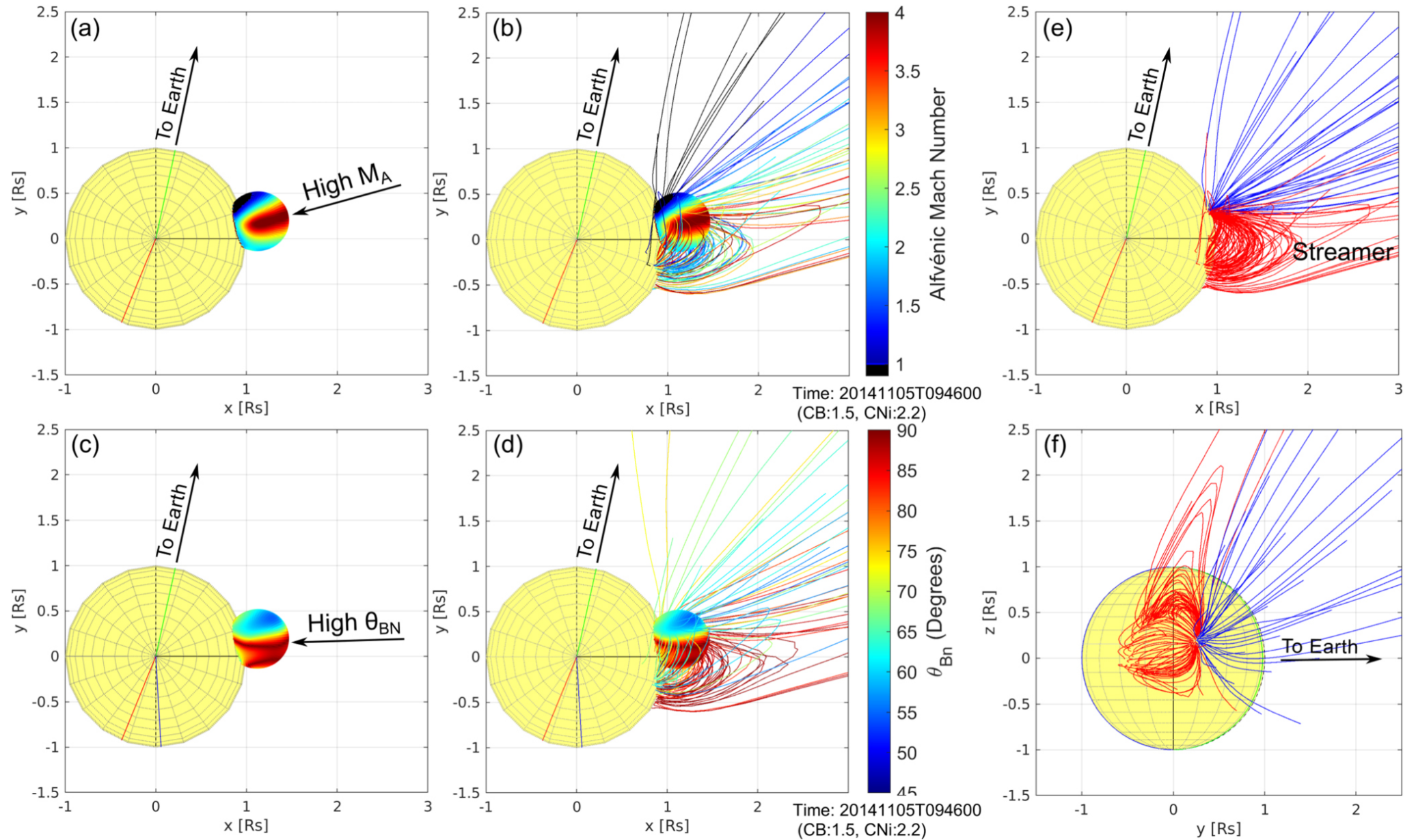
Figure 4. from Coronal Conditions for the Occurrence of Type II Radio Bursts null 2021 APJ 913 99 doi:10.3847/1538-4357/abf435 https://dx.doi.org/10.3847/1538-4357/abf435 © 2021. The Author(s). Published by the American Astronomical Society.
