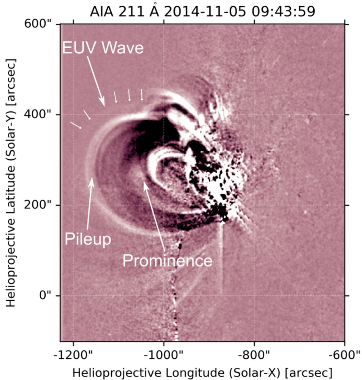
Figure 1. from Coronal Conditions for the Occurrence of Type II Radio Bursts null 2021 APJ 913 99 doi:10.3847/1538-4357/abf435 https://dx.doi.org/10.3847/1538-4357/abf435 © 2021. The Author(s). Published by the American Astronomical Society.
