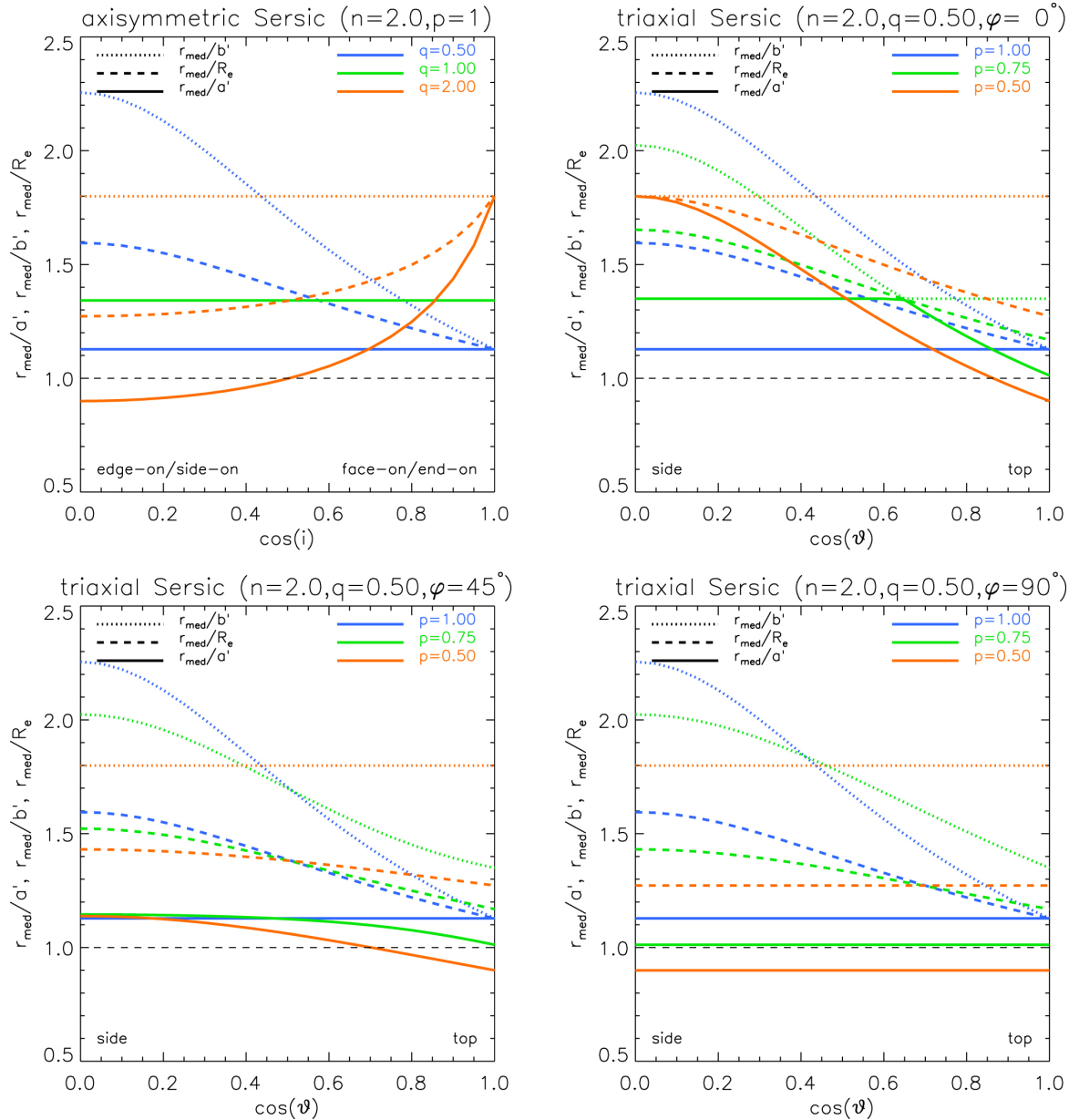
Figure 3. from Deprojecting Sérsic Profiles for Arbitrary Triaxial Shapes: Robust Measures of Intrinsic and Projected Galaxy Sizes null 2021 APJ 914 45 doi:10.3847/1538-4357/abf047 https://dx.doi.org/10.3847/1538-4357/abf047
