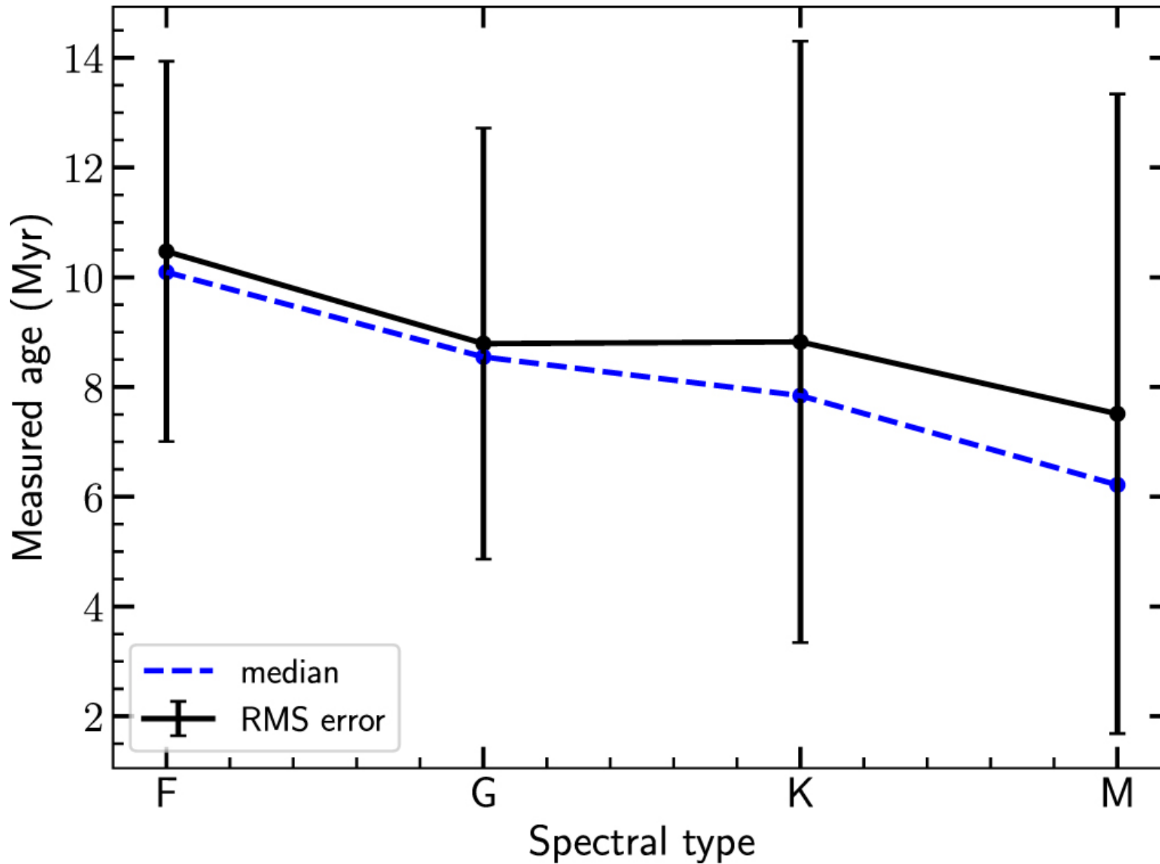
Figure 10. from Undetected Binary Stars Cause an Observed Mass-dependent Age Gradient in Upper Scorpius null 2021 APJ 912 137 doi:10.3847/1538-4357/abf044 https://dx.doi.org/10.3847/1538-4357/abf044 © 2021. The American Astronomical Society. All rights reserved.
