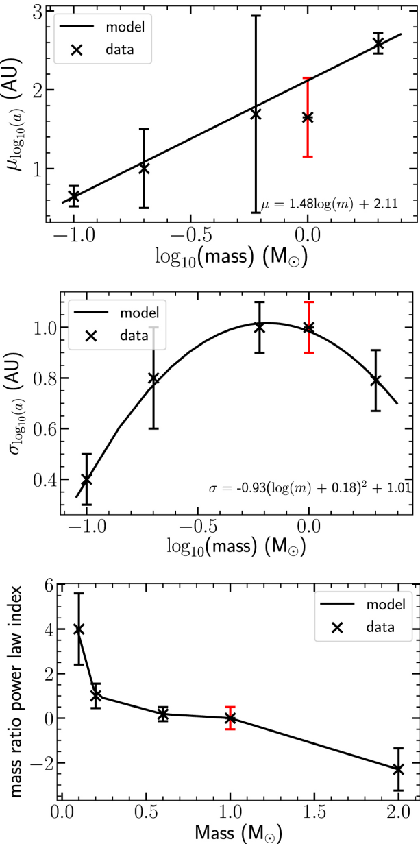
Figure 1. from Undetected Binary Stars Cause an Observed Mass-dependent Age Gradient in Upper Scorpius null 2021 APJ 912 137 doi:10.3847/1538-4357/abf044 https://dx.doi.org/10.3847/1538-4357/abf044 © 2021. The American Astronomical Society. All rights reserved.
