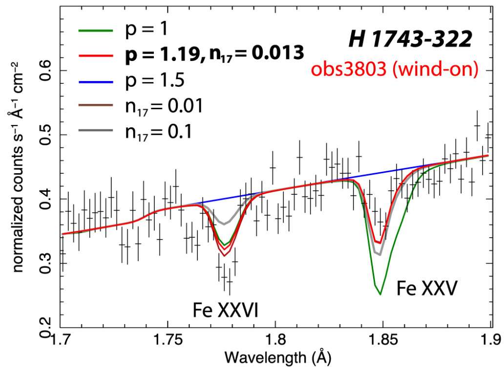
Figure 9. from Modeling Magnetic Disk Wind State Transitions in Black Hole X-Ray Binaries null 2021 APJ 912 86 doi:10.3847/1538-4357/abedaf https://dx.doi.org/10.3847/1538-4357/abedaf © 2021. The American Astronomical Society. All rights reserved.
