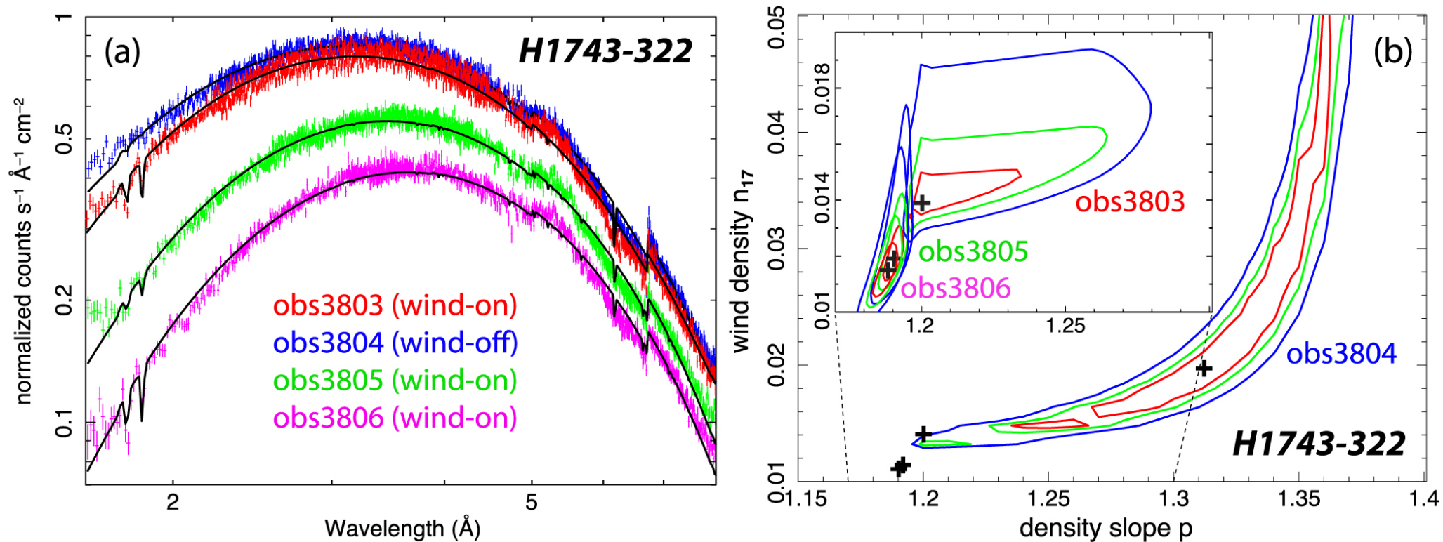
Figure 5. from Modeling Magnetic Disk Wind State Transitions in Black Hole X-Ray Binaries null 2021 APJ 912 86 doi:10.3847/1538-4357/abedaf https://dx.doi.org/10.3847/1538-4357/abedaf © 2021. The American Astronomical Society. All rights reserved.
