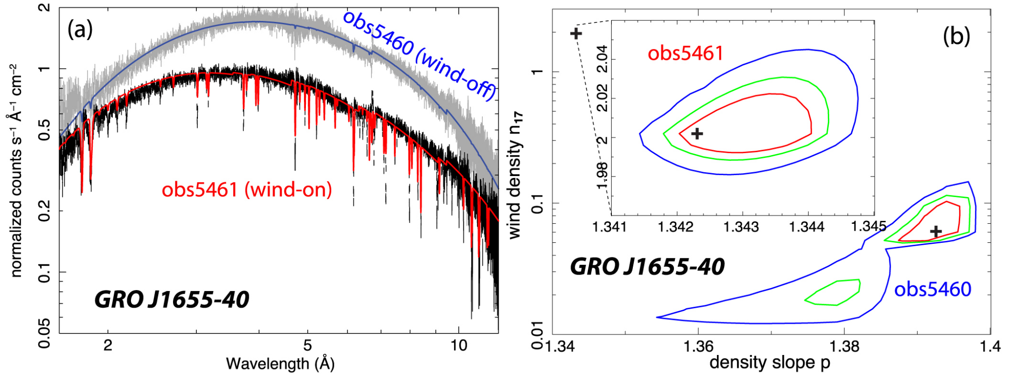
Figure 4. from Modeling Magnetic Disk Wind State Transitions in Black Hole X-Ray Binaries null 2021 APJ 912 86 doi:10.3847/1538-4357/abedaf https://dx.doi.org/10.3847/1538-4357/abedaf © 2021. The American Astronomical Society. All rights reserved.
