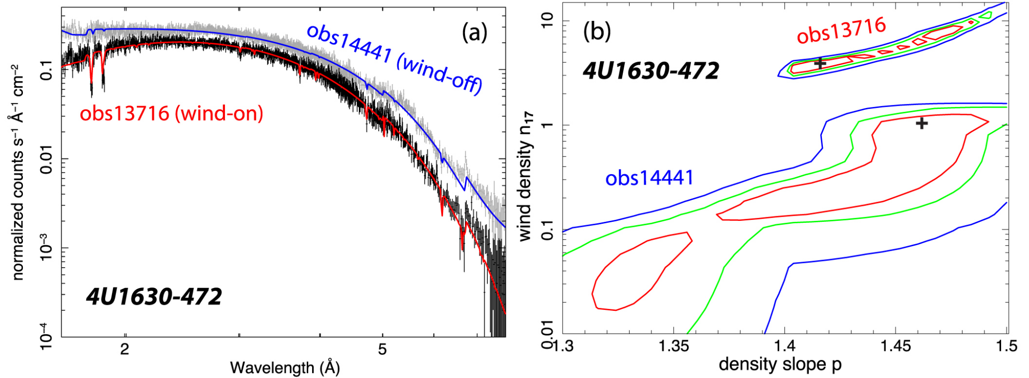
Figure 3. from Modeling Magnetic Disk Wind State Transitions in Black Hole X-Ray Binaries null 2021 APJ 912 86 doi:10.3847/1538-4357/abedaf https://dx.doi.org/10.3847/1538-4357/abedaf © 2021. The American Astronomical Society. All rights reserved.
