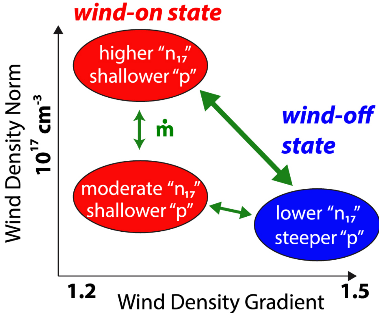
Figure 19. from Modeling Magnetic Disk Wind State Transitions in Black Hole X-Ray Binaries null 2021 APJ 912 86 doi:10.3847/1538-4357/abedaf https://dx.doi.org/10.3847/1538-4357/abedaf © 2021. The American Astronomical Society. All rights reserved.
