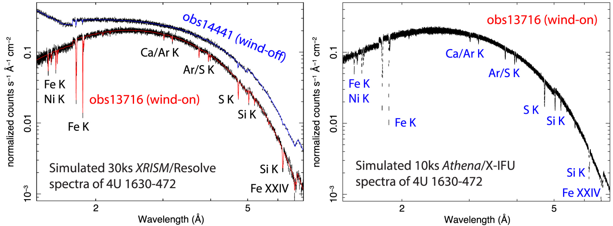
Figure 18. from Modeling Magnetic Disk Wind State Transitions in Black Hole X-Ray Binaries null 2021 APJ 912 86 doi:10.3847/1538-4357/abedaf https://dx.doi.org/10.3847/1538-4357/abedaf © 2021. The American Astronomical Society. All rights reserved.
