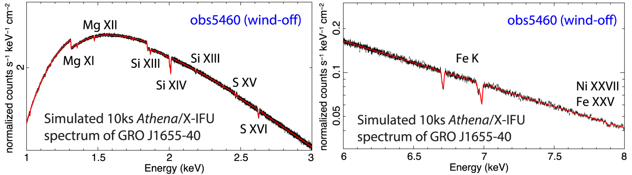
Figure 16. from Modeling Magnetic Disk Wind State Transitions in Black Hole X-Ray Binaries null 2021 APJ 912 86 doi:10.3847/1538-4357/abedaf https://dx.doi.org/10.3847/1538-4357/abedaf © 2021. The American Astronomical Society. All rights reserved.
