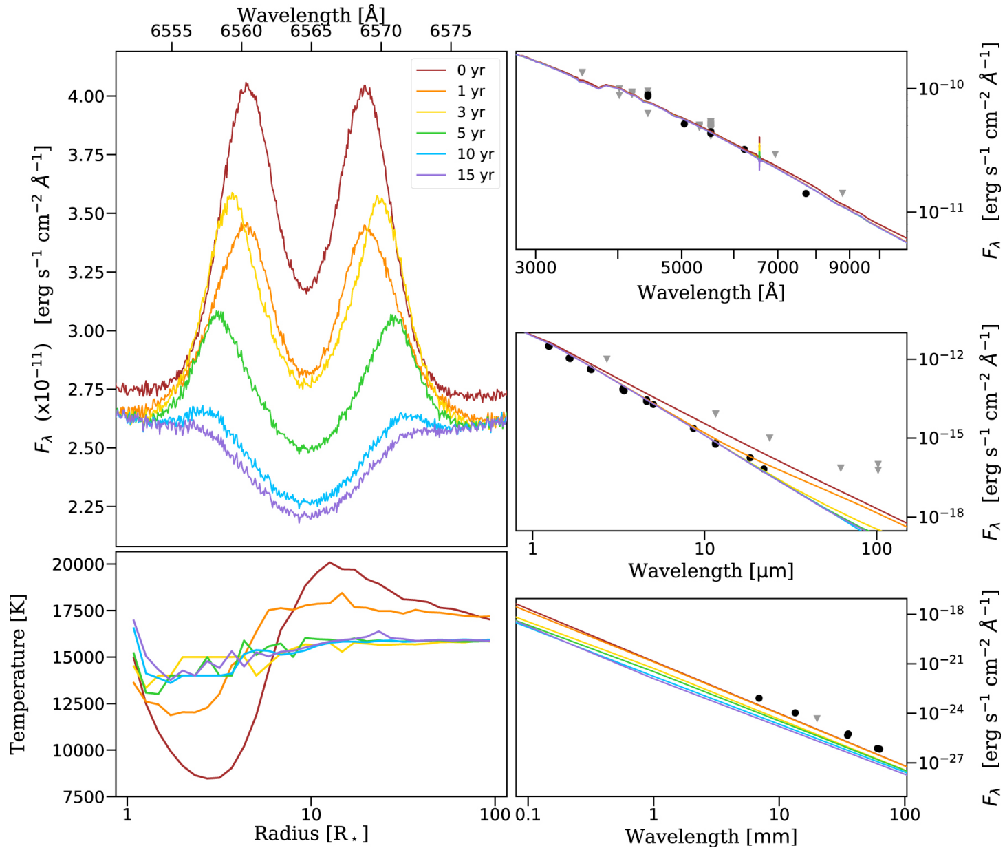
Figure 9. from The Be Star 66 Ophiuchi: 60 Years of Disk Evolution null 2021 APJ 912 76 doi:10.3847/1538-4357/abed4c https://dx.doi.org/10.3847/1538-4357/abed4c © 2021. The American Astronomical Society. All rights reserved.
