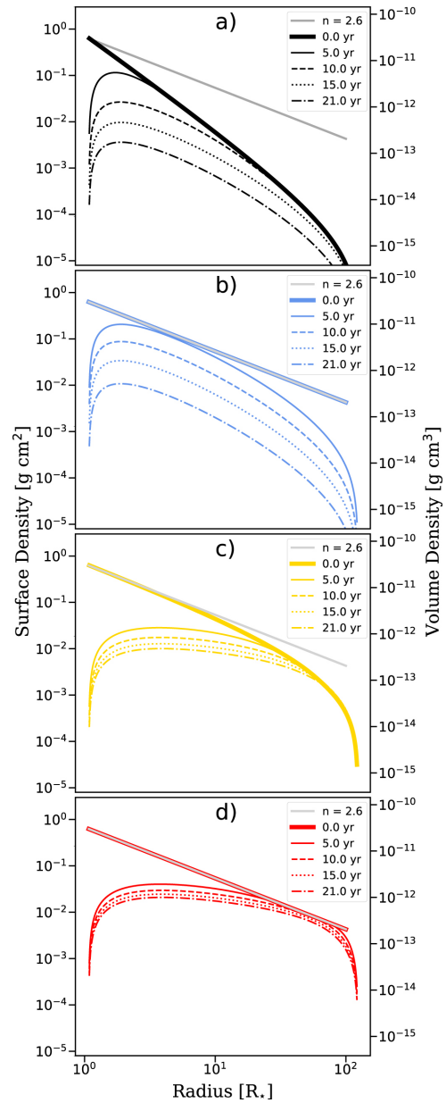
Figure 8. from The Be Star 66 Ophiuchi: 60 Years of Disk Evolution null 2021 APJ 912 76 doi:10.3847/1538-4357/abed4c https://dx.doi.org/10.3847/1538-4357/abed4c © 2021. The American Astronomical Society. All rights reserved.
