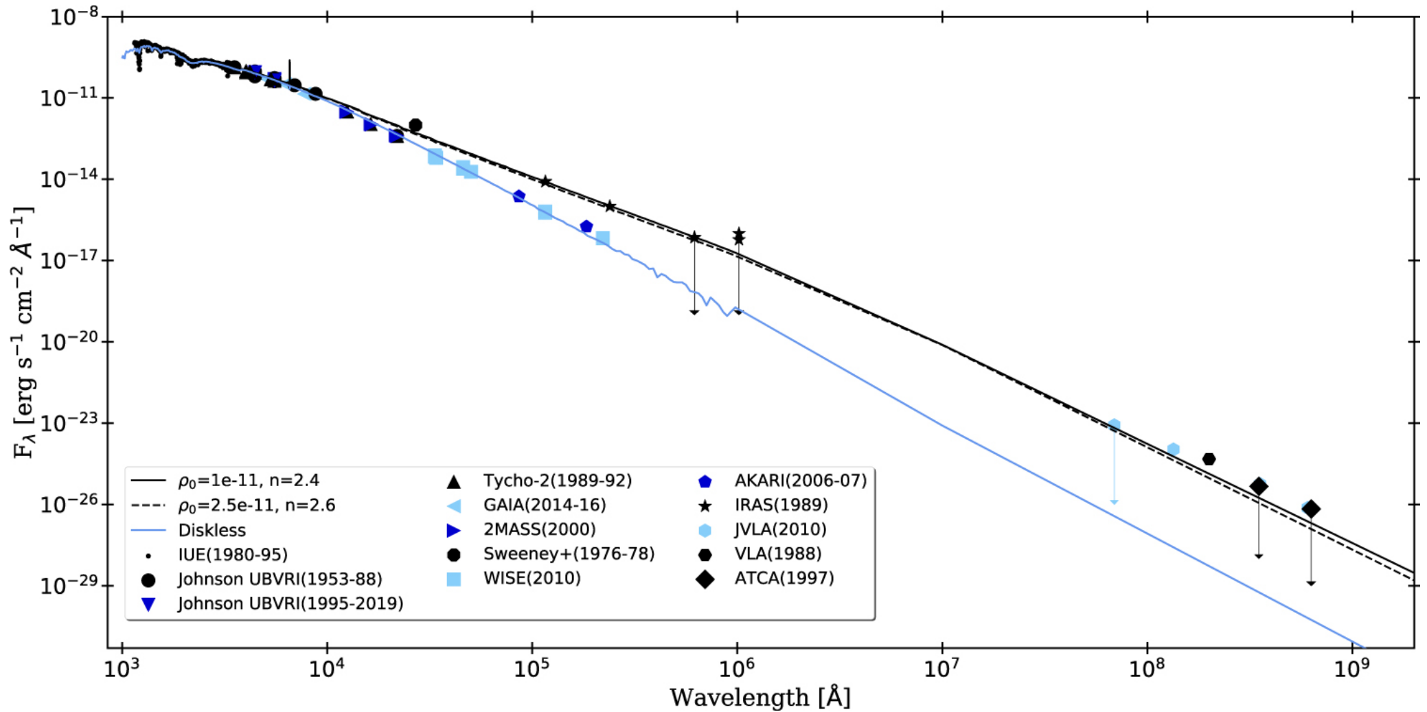
Figure 6. from The Be Star 66 Ophiuchi: 60 Years of Disk Evolution null 2021 APJ 912 76 doi:10.3847/1538-4357/abed4c https://dx.doi.org/10.3847/1538-4357/abed4c © 2021. The American Astronomical Society. All rights reserved.
