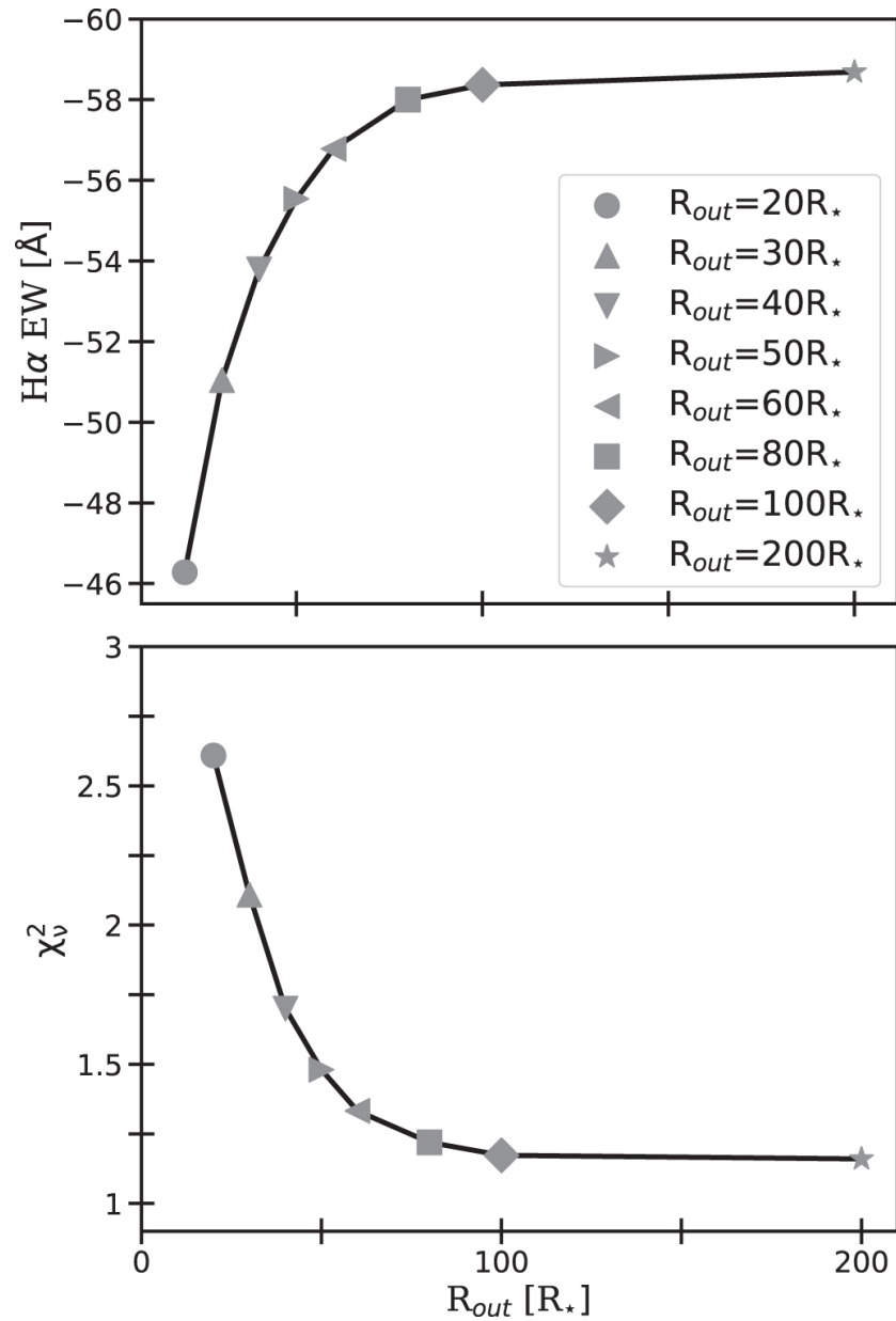
Figure 5. from The Be Star 66 Ophiuchi: 60 Years of Disk Evolution null 2021 APJ 912 76 doi:10.3847/1538-4357/abed4c https://dx.doi.org/10.3847/1538-4357/abed4c © 2021. The American Astronomical Society. All rights reserved.
