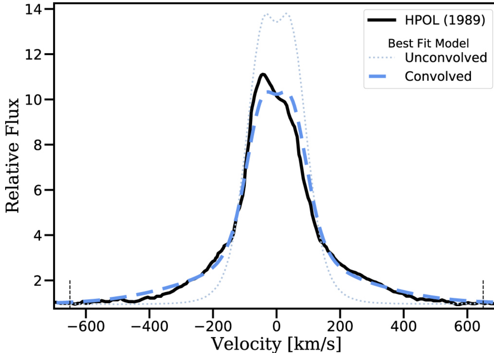
Figure 4. from The Be Star 66 Ophiuchi: 60 Years of Disk Evolution null 2021 APJ 912 76 doi:10.3847/1538-4357/abed4c https://dx.doi.org/10.3847/1538-4357/abed4c © 2021. The American Astronomical Society. All rights reserved.
