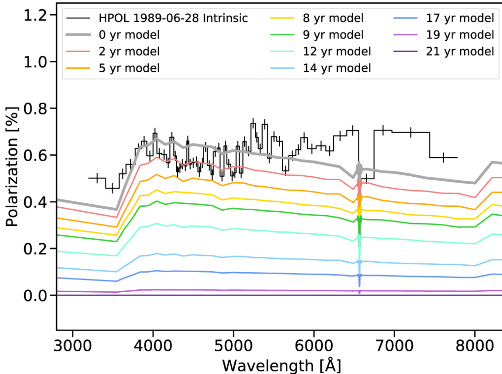
Figure 15. from The Be Star 66 Ophiuchi: 60 Years of Disk Evolution null 2021 APJ 912 76 doi:10.3847/1538-4357/abed4c https://dx.doi.org/10.3847/1538-4357/abed4c © 2021. The American Astronomical Society. All rights reserved.
