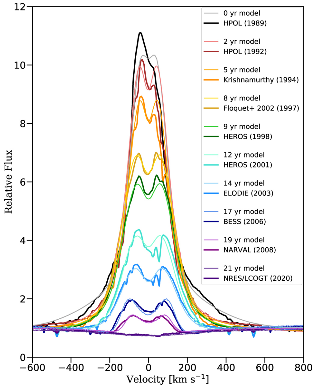
Figure 14. from The Be Star 66 Ophiuchi: 60 Years of Disk Evolution null 2021 APJ 912 76 doi:10.3847/1538-4357/abed4c https://dx.doi.org/10.3847/1538-4357/abed4c © 2021. The American Astronomical Society. All rights reserved.
