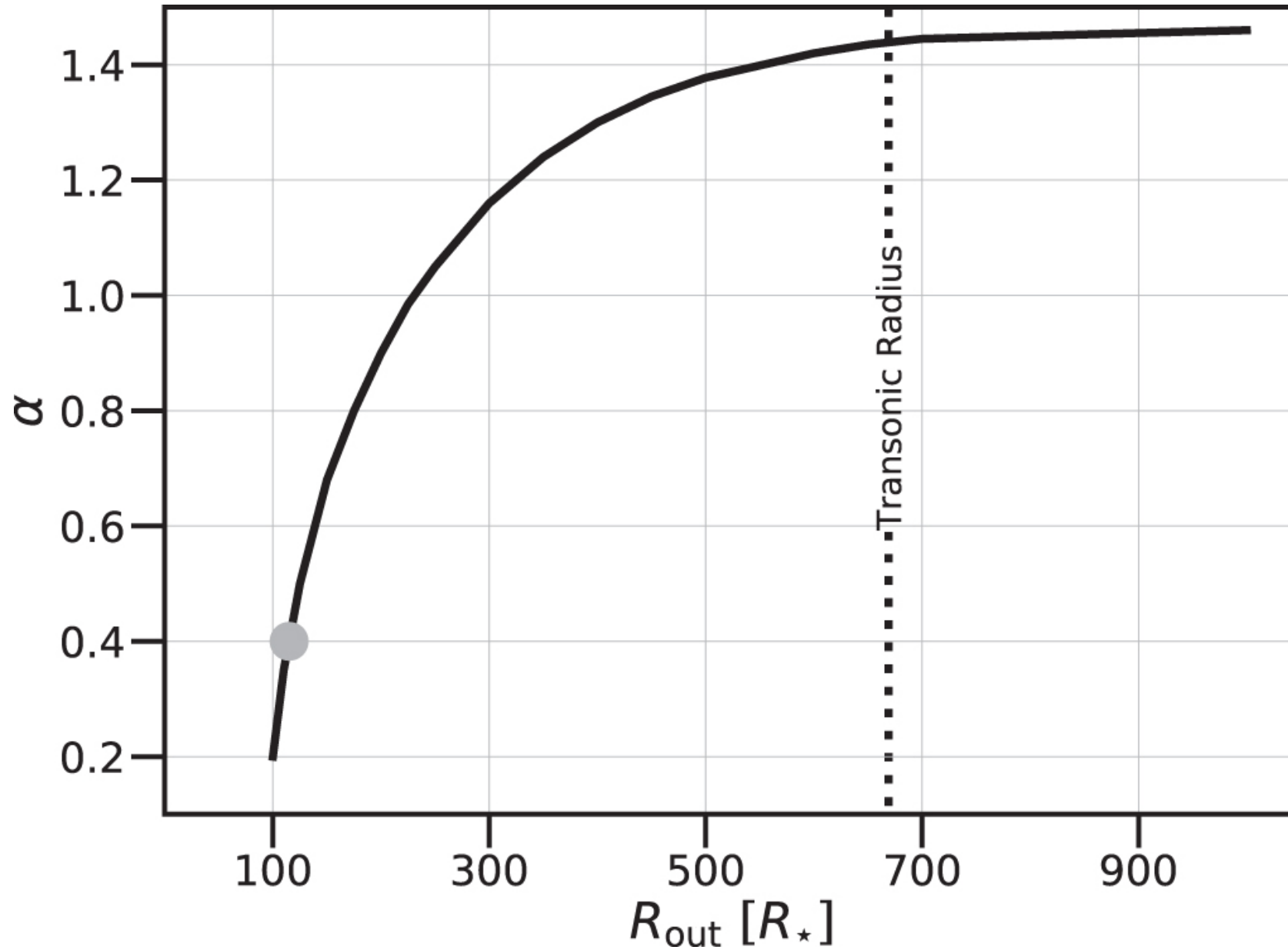
Figure 13. from The Be Star 66 Ophiuchi: 60 Years of Disk Evolution null 2021 APJ 912 76 doi:10.3847/1538-4357/abed4c https://dx.doi.org/10.3847/1538-4357/abed4c © 2021. The American Astronomical Society. All rights reserved.
