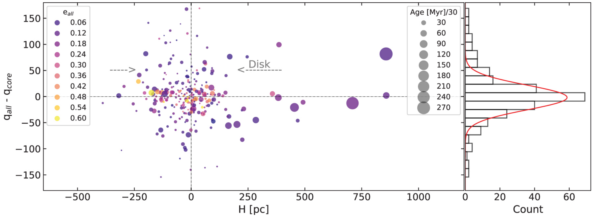
Figure 9. from Deciphering Star Cluster Evolution by Shape Morphology null 2021 APJ 912 5 doi:10.3847/1538-4357/abec3e https://dx.doi.org/10.3847/1538-4357/abec3e © 2021. The American Astronomical Society. All rights reserved.
