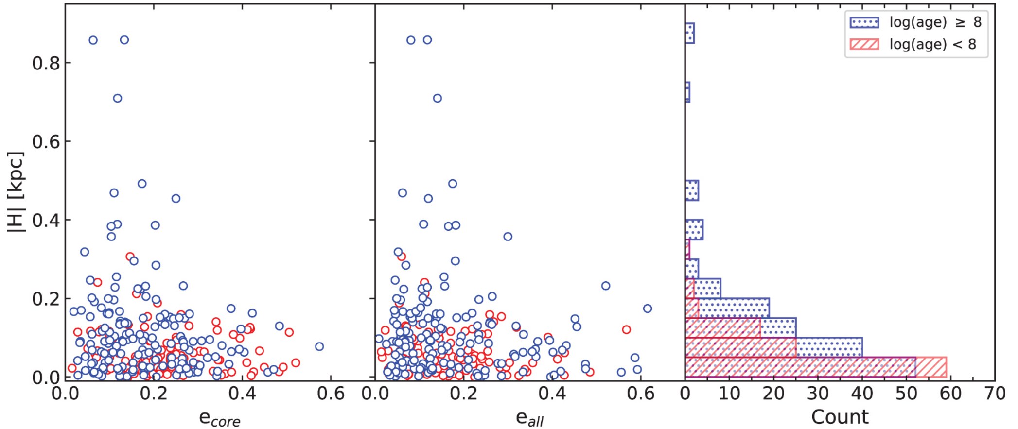
Figure 7. from Deciphering Star Cluster Evolution by Shape Morphology null 2021 APJ 912 5 doi:10.3847/1538-4357/abec3e https://dx.doi.org/10.3847/1538-4357/abec3e © 2021. The American Astronomical Society. All rights reserved.
