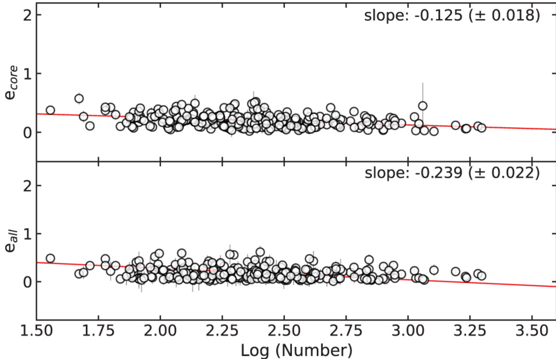
Figure 5. from Deciphering Star Cluster Evolution by Shape Morphology null 2021 APJ 912 5 doi:10.3847/1538-4357/abec3e https://dx.doi.org/10.3847/1538-4357/abec3e © 2021. The American Astronomical Society. All rights reserved.
