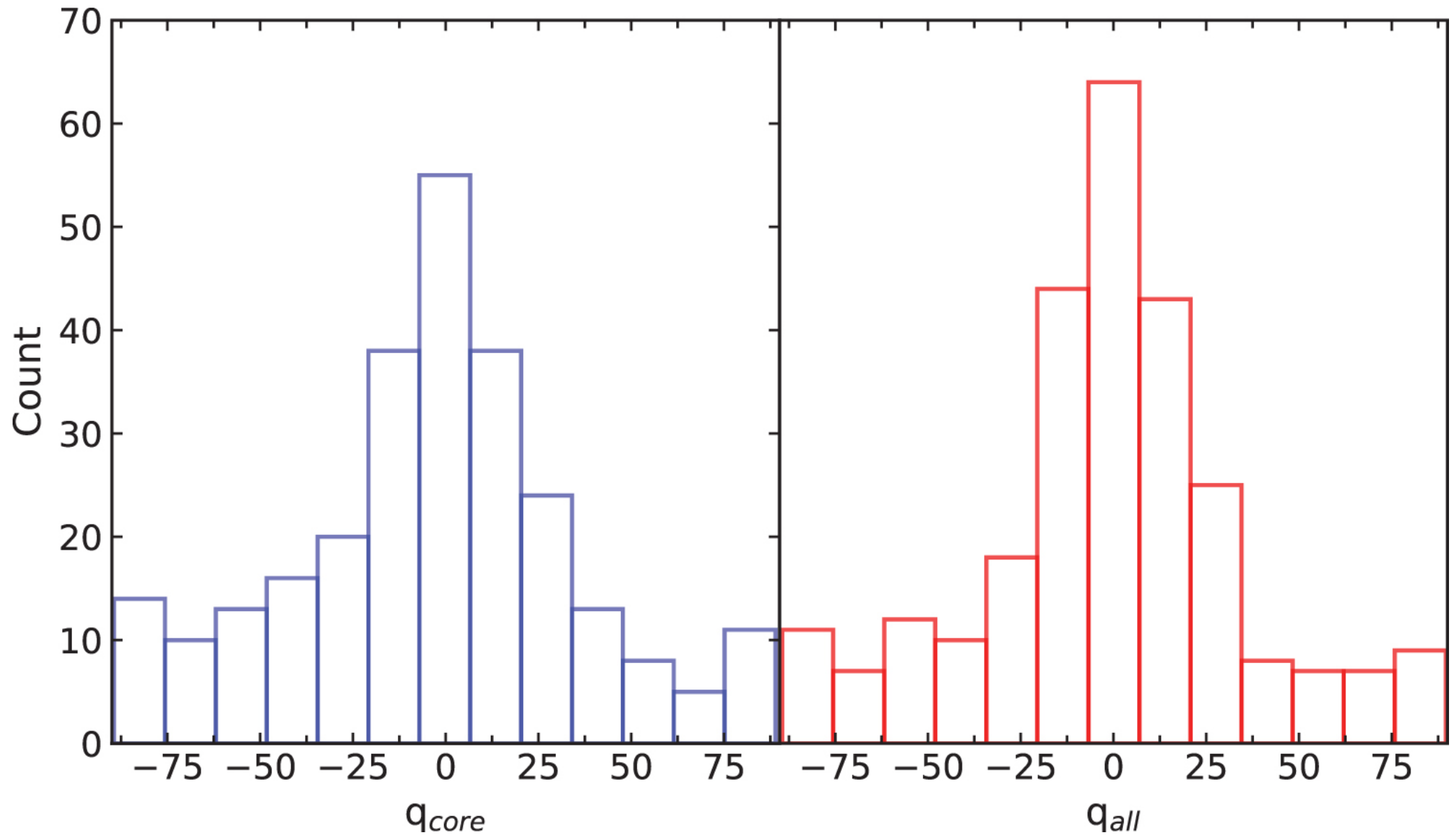
Figure 3. from Deciphering Star Cluster Evolution by Shape Morphology null 2021 APJ 912 5 doi:10.3847/1538-4357/abec3e https://dx.doi.org/10.3847/1538-4357/abec3e © 2021. The American Astronomical Society. All rights reserved.
