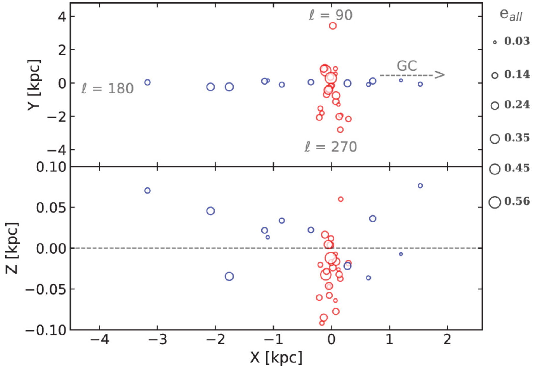
Figure 10. from Deciphering Star Cluster Evolution by Shape Morphology null 2021 APJ 912 5 doi:10.3847/1538-4357/abec3e https://dx.doi.org/10.3847/1538-4357/abec3e © 2021. The American Astronomical Society. All rights reserved.
