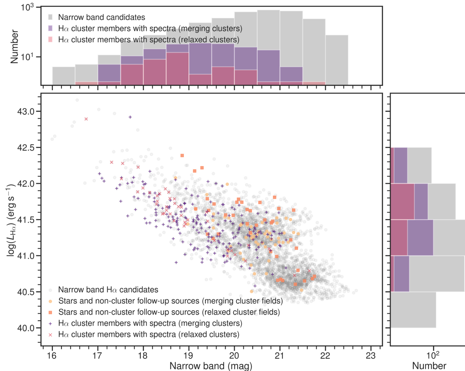
Figure 9. from ENISALA. II. Distinct Star Formation and Active Galactic Nucleus Activity in Merging and Relaxed Galaxy Clusters null 2021 APJ 912 55 doi:10.3847/1538-4357/abe7f8 https://dx.doi.org/10.3847/1538-4357/abe7f8 © 2021. The American Astronomical Society. All rights reserved.
