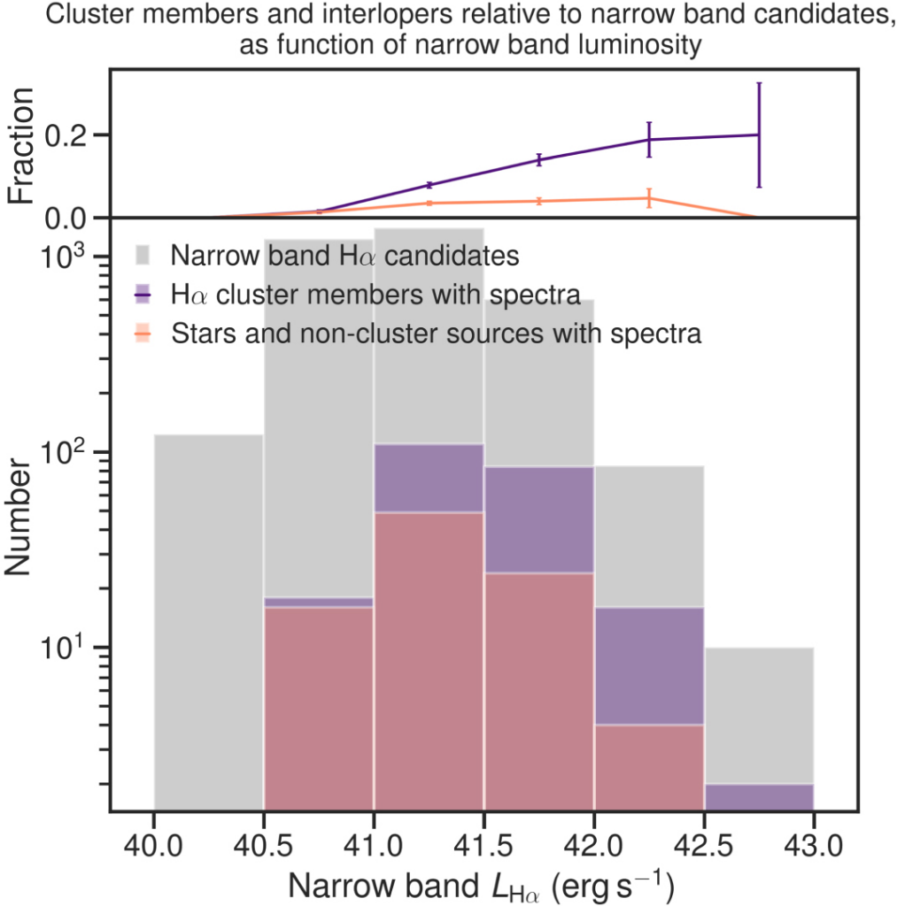
Figure 8. from ENISALA. II. Distinct Star Formation and Active Galactic Nucleus Activity in Merging and Relaxed Galaxy Clusters null 2021 APJ 912 55 doi:10.3847/1538-4357/abe7f8 https://dx.doi.org/10.3847/1538-4357/abe7f8 © 2021. The American Astronomical Society. All rights reserved.
